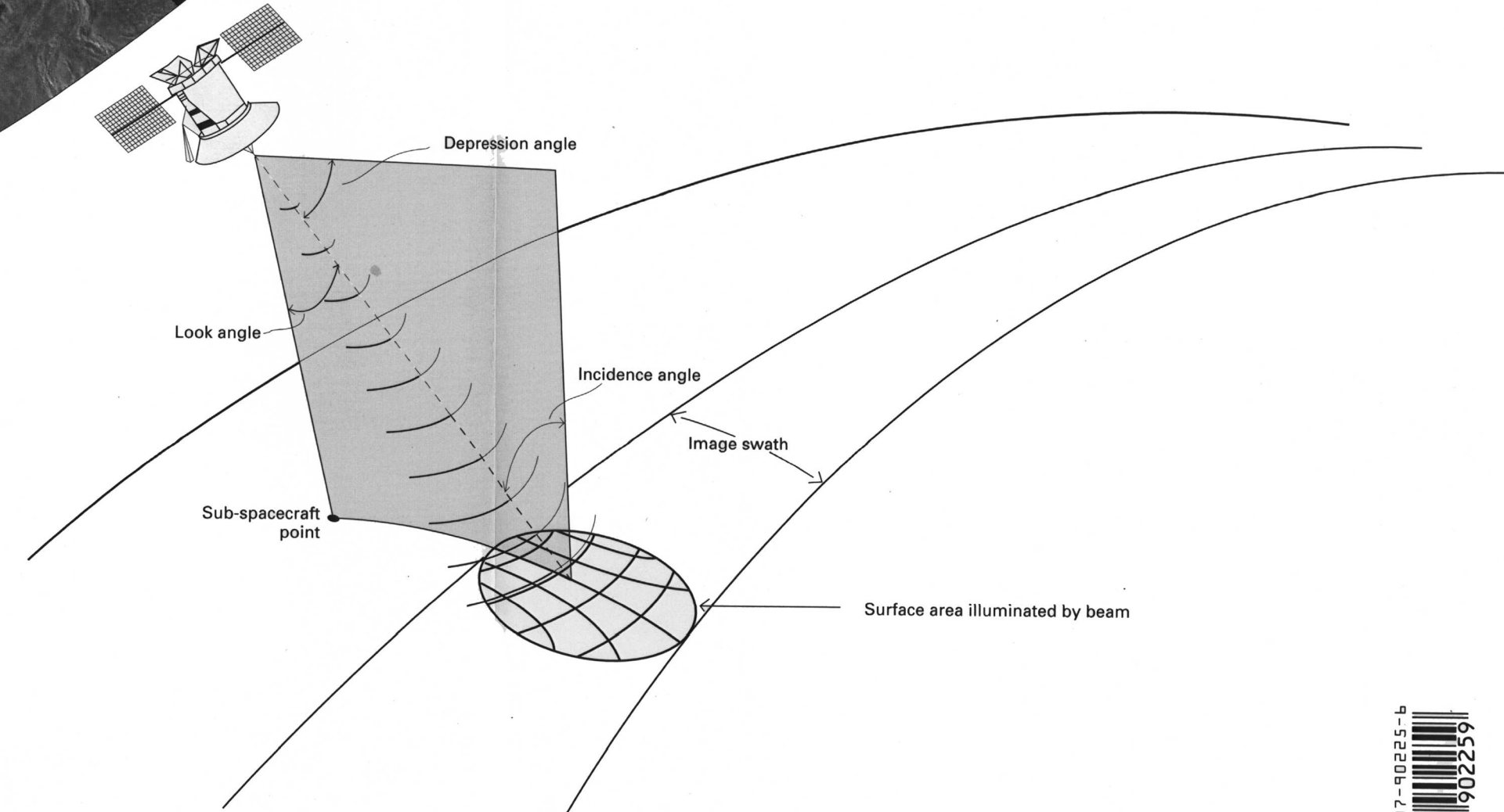
Figure 2. Geometry of the Magellan Synthetic Aperture Radar (SAR) footprint and terminology.
