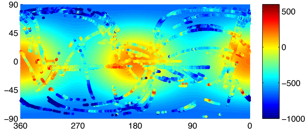
fit-triaxial-norot-no-trans.rdf, rms error=213.7611 a,b,c =2575207.1431,2574666.8445,2574354.8425 offsets:0,0,0
