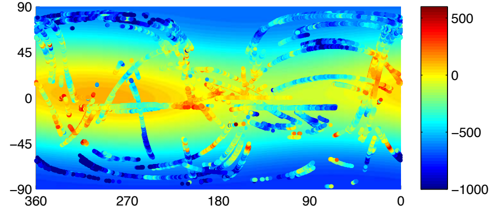
fit-biaxial.rdf, rms error=236.0905 a,b,c =2575007.4602,2575007.4602,2574310.5525 offsets:47.6058,96.4946,50.7326
