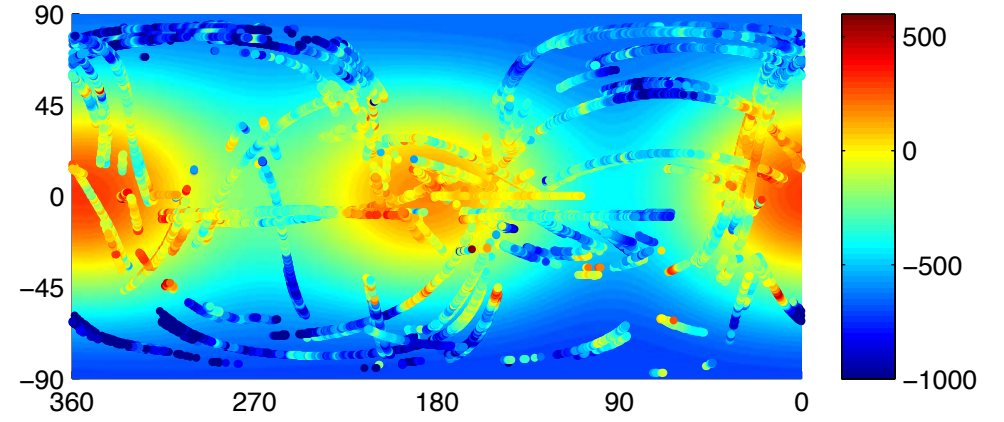
fit-triaxial-norot.rdf, rms error=206.0904 a,b,c =2575238.959,2574685.5791,2574324.1054 offsets:64.3687,102.3637,38.3817
