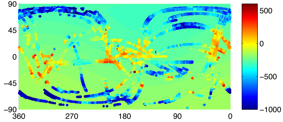
fit-sphere.rdf, rms error=330.008 a,b,c =2574768.5873,2574768.5873,2574768.5873 offsets:24.9727,19.7678,-67.4504
