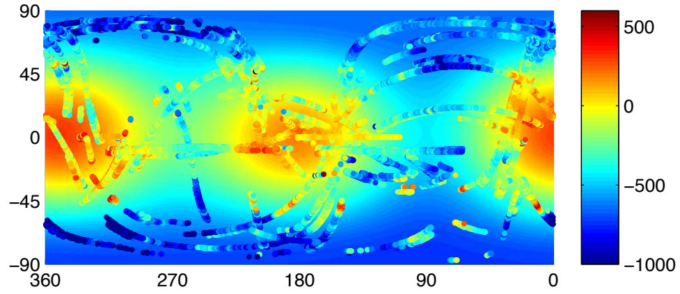
fit-triaxial.rdf, rms error=205.5351 a,b,c =2575239.6402,2574686.4318,2574318.2344 offsets:69.1582,109.7427,41.4551
