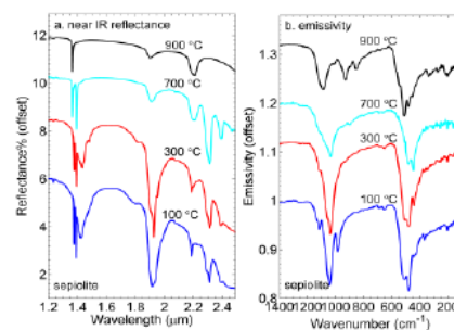
Figure 2. (a) Near IR reflectance and (b) TIR emissivity spectra of heated sepiolite. At 900 °C, sepiolite displays spectral bands at 1.9 and 2.2 \mu\text{m} that are diagnostic of phyllosilicates, while its TIR spectrum is already dominated by spectral bands of enstatite.
