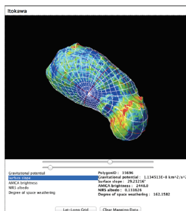
Fig. 1 A snapshot of 3D-GIS displaying Itokawa with a slope map
