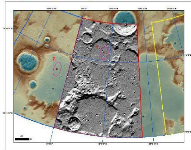
Figure 2. Hill-shaded relief map. Azimuth 315^\circ , solar elevation angle 45^\circ (background – color shaded relief from “GLD100”)
