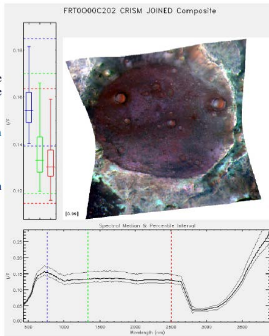
Figure 3 (Left). FRT0000C202 MTRDR three-panel composite. The spectral MTRDR data product incorporates all of the VNIR and IR detector-specific data processing (Figure 1, Figure 2) and the VNIR/IR sensor space transform to spatially align the constituent image cubes. The map projection is consistent with the ‘rolling equirectangular’ MRO standard. Note that the MTRDR RGB composite combines bands that source from both the VNIR (B: ~770 nm) and IR (G: ~1330 nm; R:~2510 nm) detectors.
