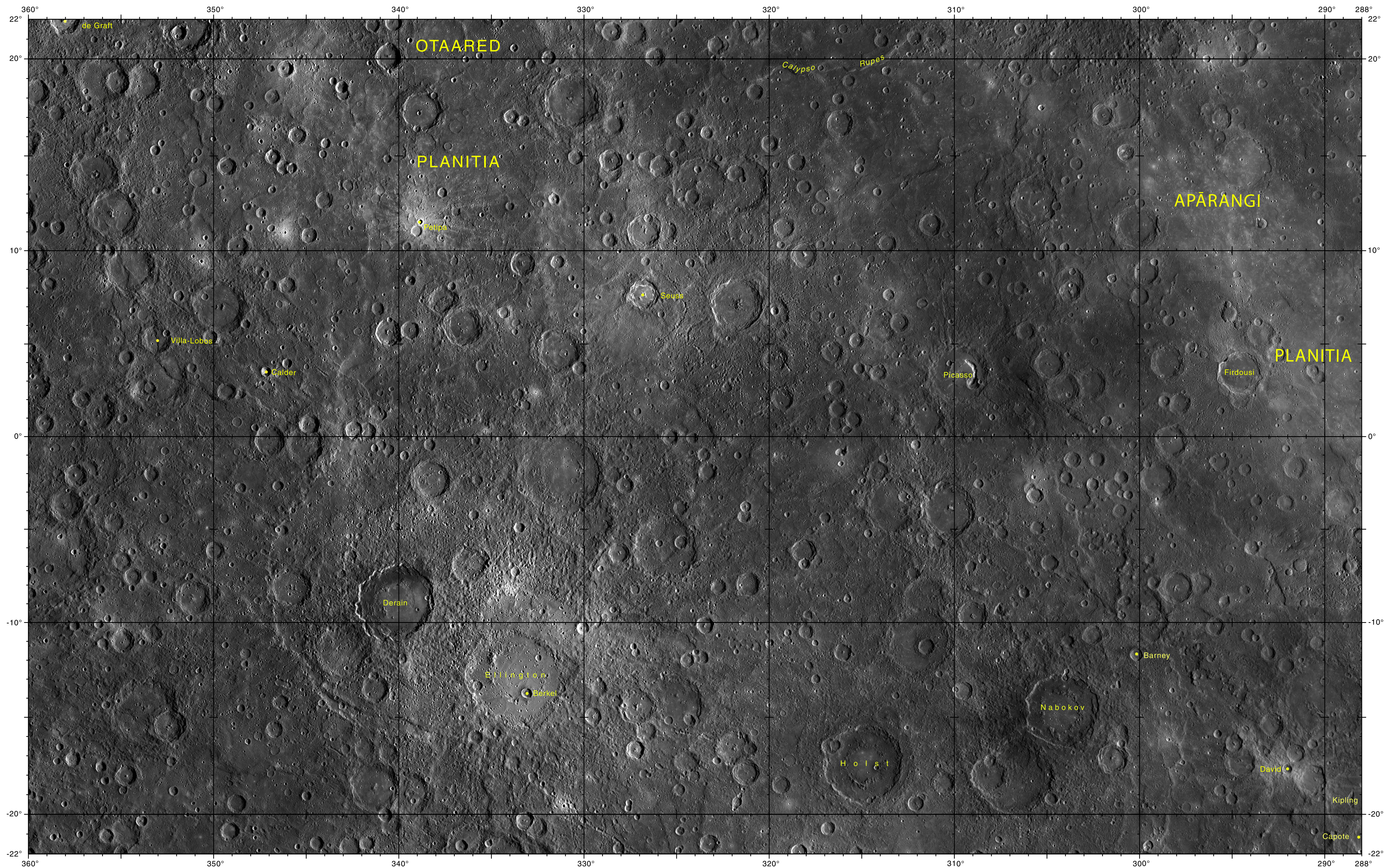
Map of the H-10 (Derain) Quadrangle of Mercury
